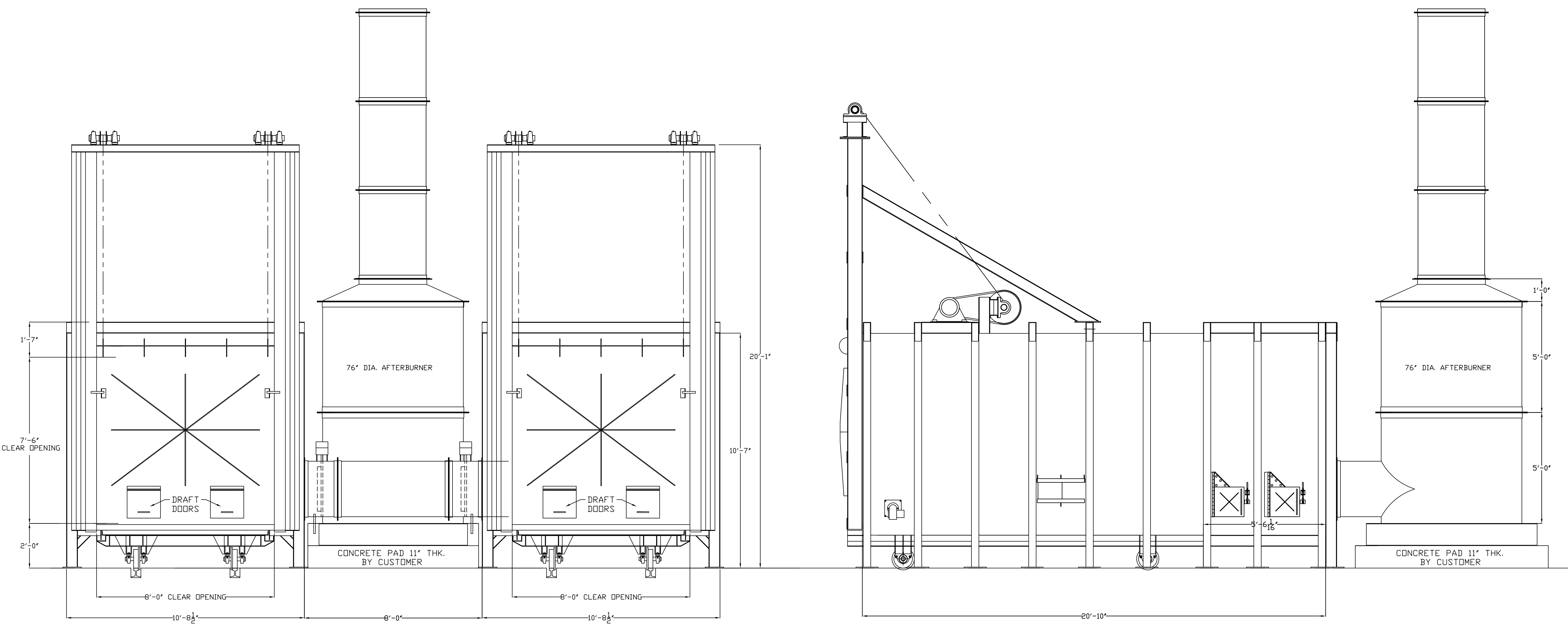
FRONT VIEW
